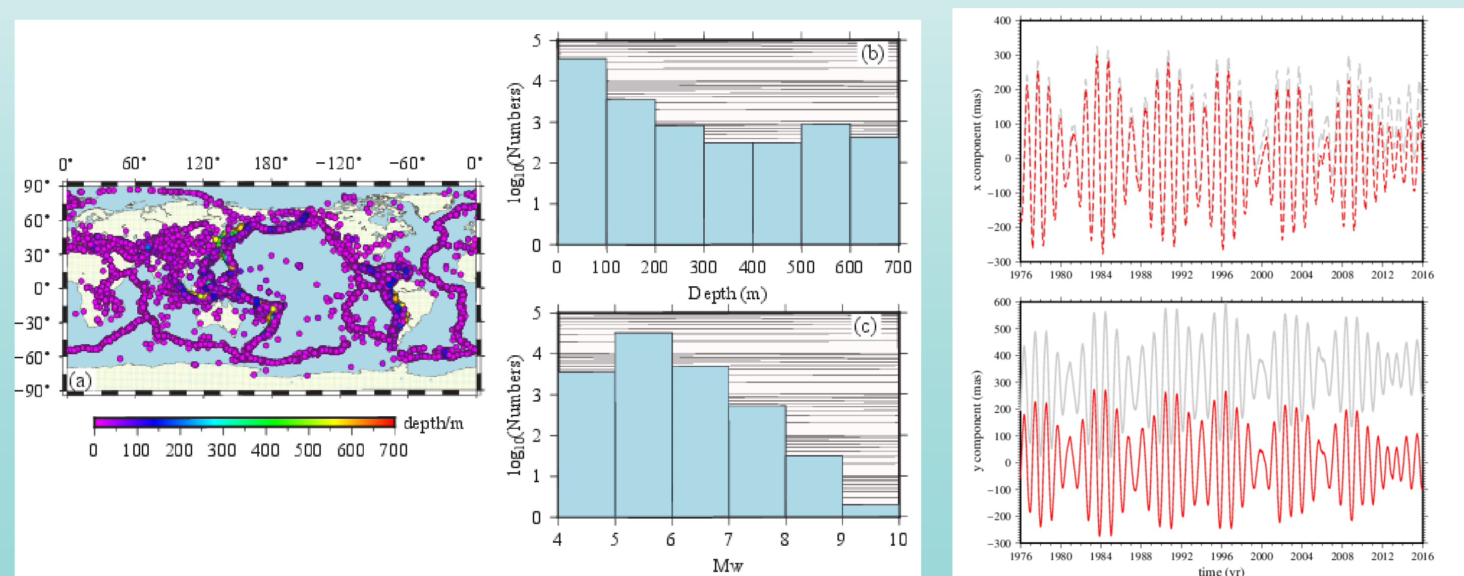
Figure 1: Focal mechanisms from GCMT catalog during 1976 to 2016 (left) and observed polar motion time series adopted from IERS 14 C04 solutions (right).
