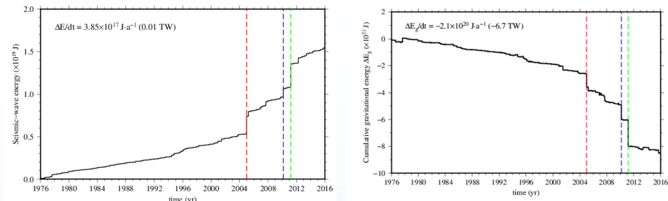
Figure 4: Cumulative changes in seismic-wave energy and E_g from 1976 to 2016
