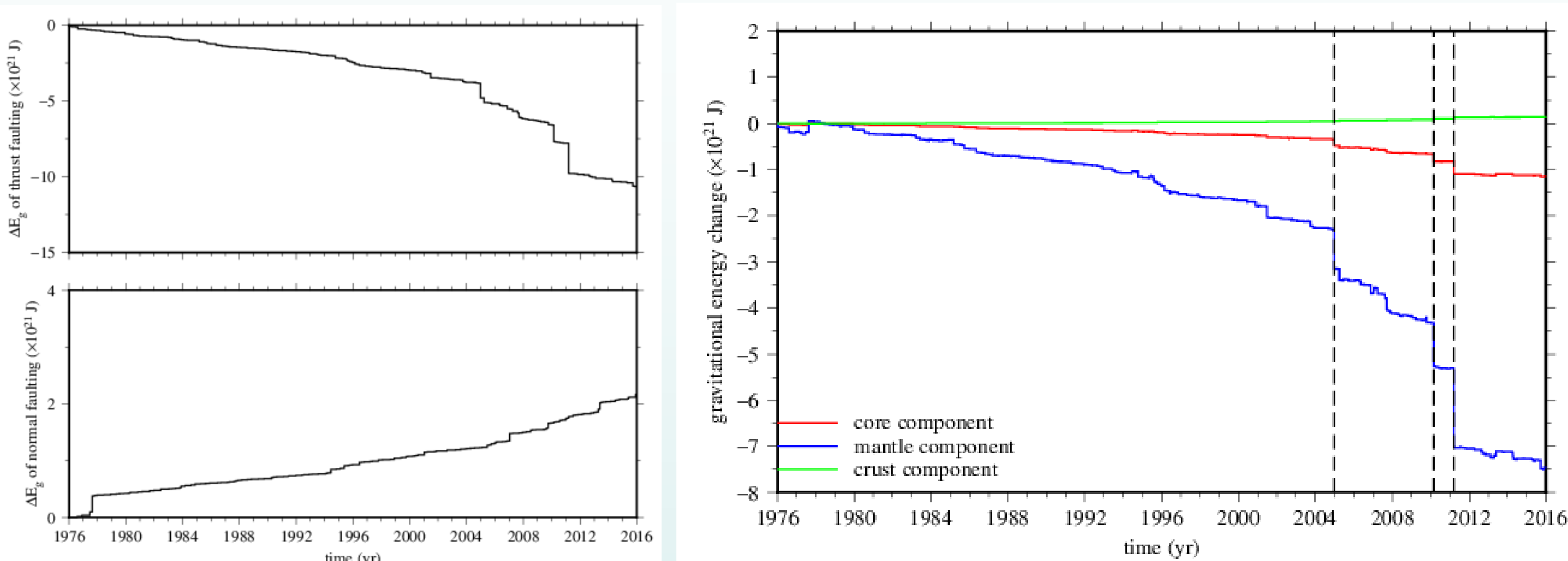
Figure 5: Cumulative changes in E_g for two-types faulting (left) and for different parts of the Earth from 1976 to 2016
