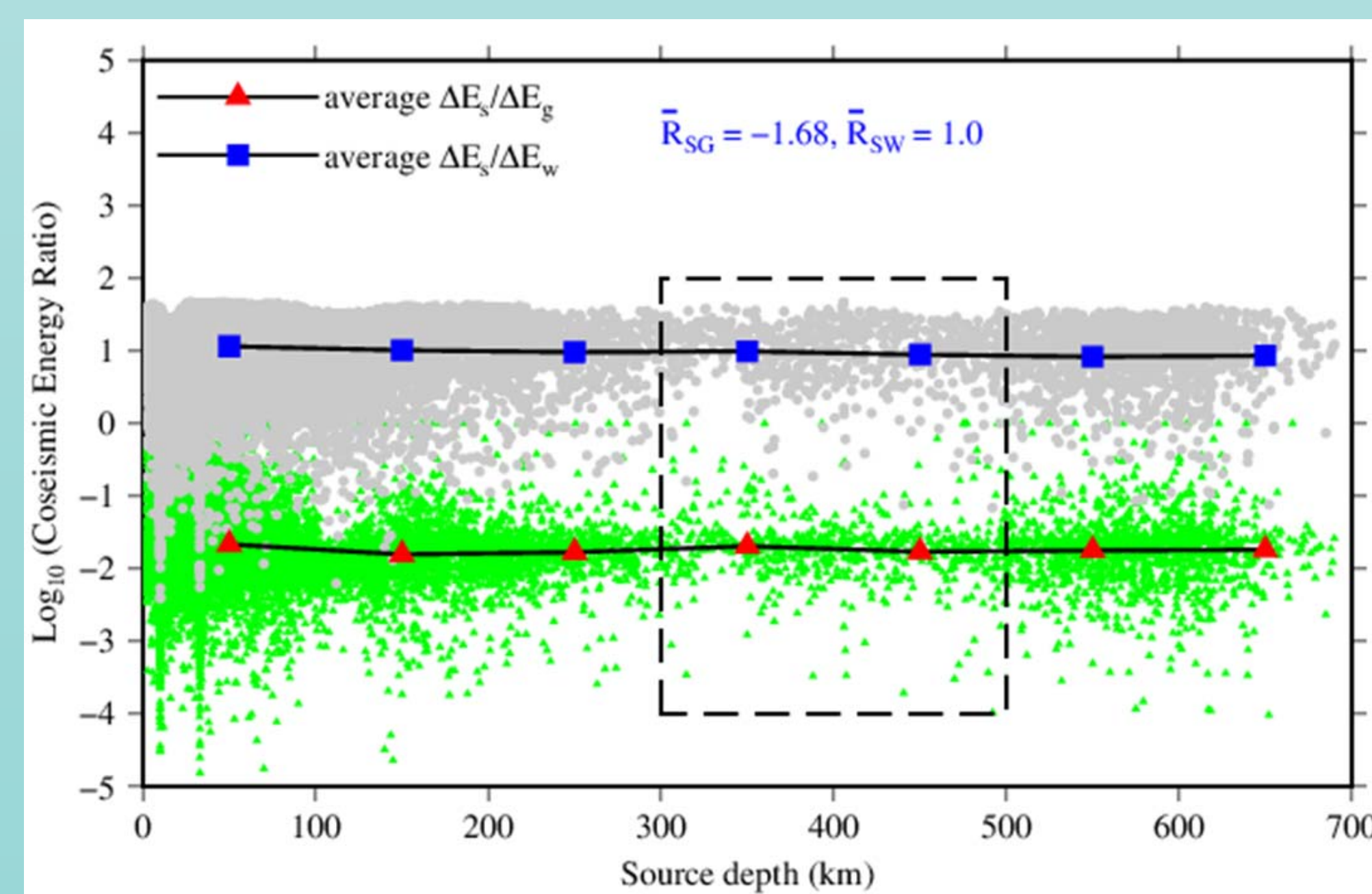
Figure 7: Energy ratio for coseismic changes in E_g , E_s and seismic-wave energy
