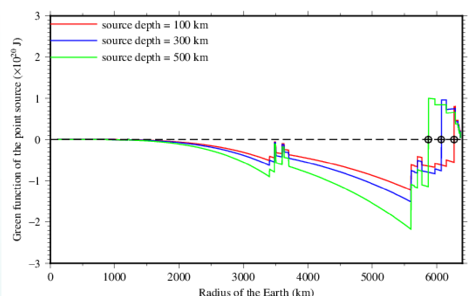
Figure 2: Green functions of coseismic change in E_g at three different source depth.
