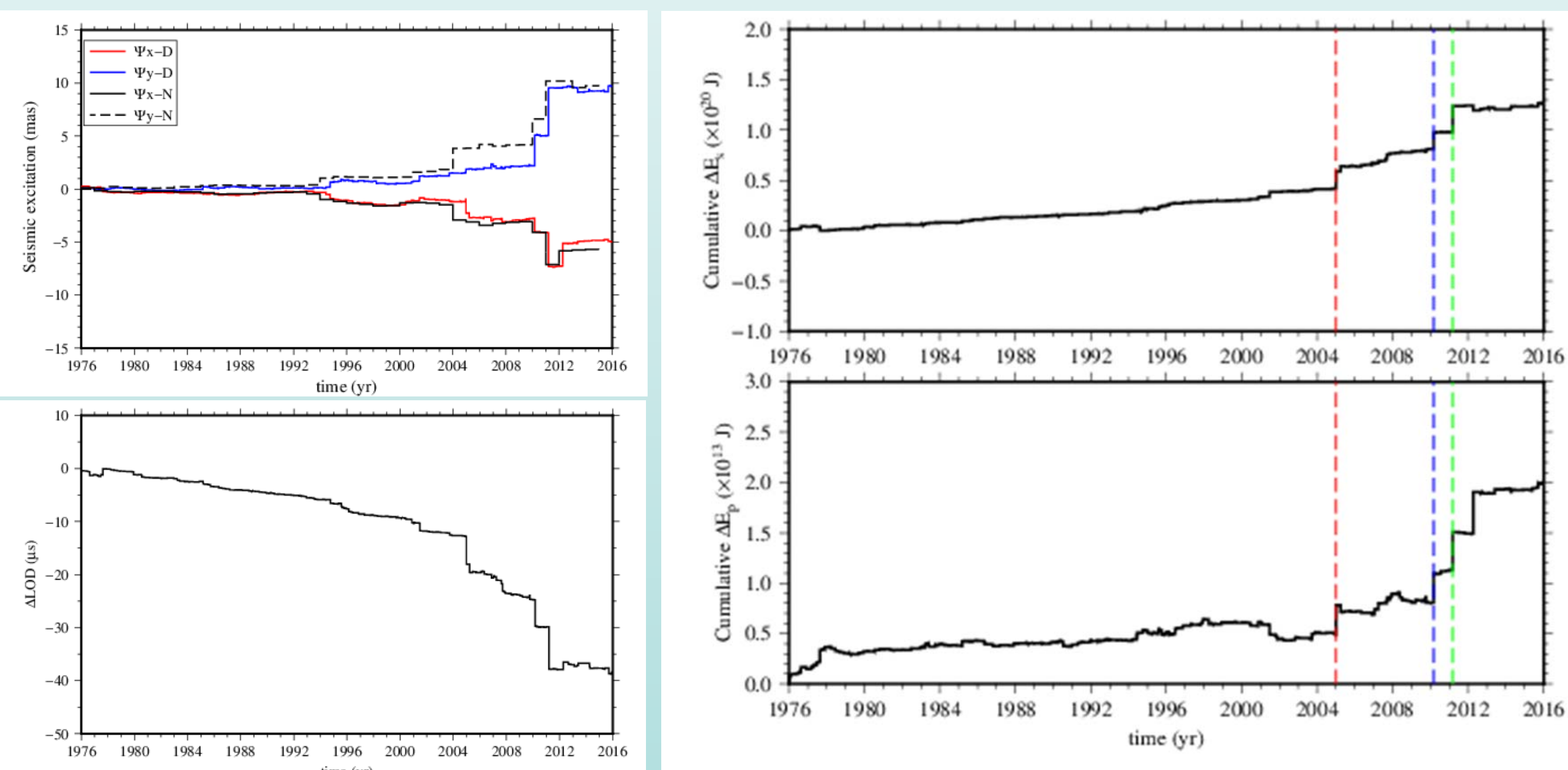
Figure 6: Cumulative changes in earthquake-excited polar motion, excess length of day and kinetic rotational energy from 1976 to 2016
