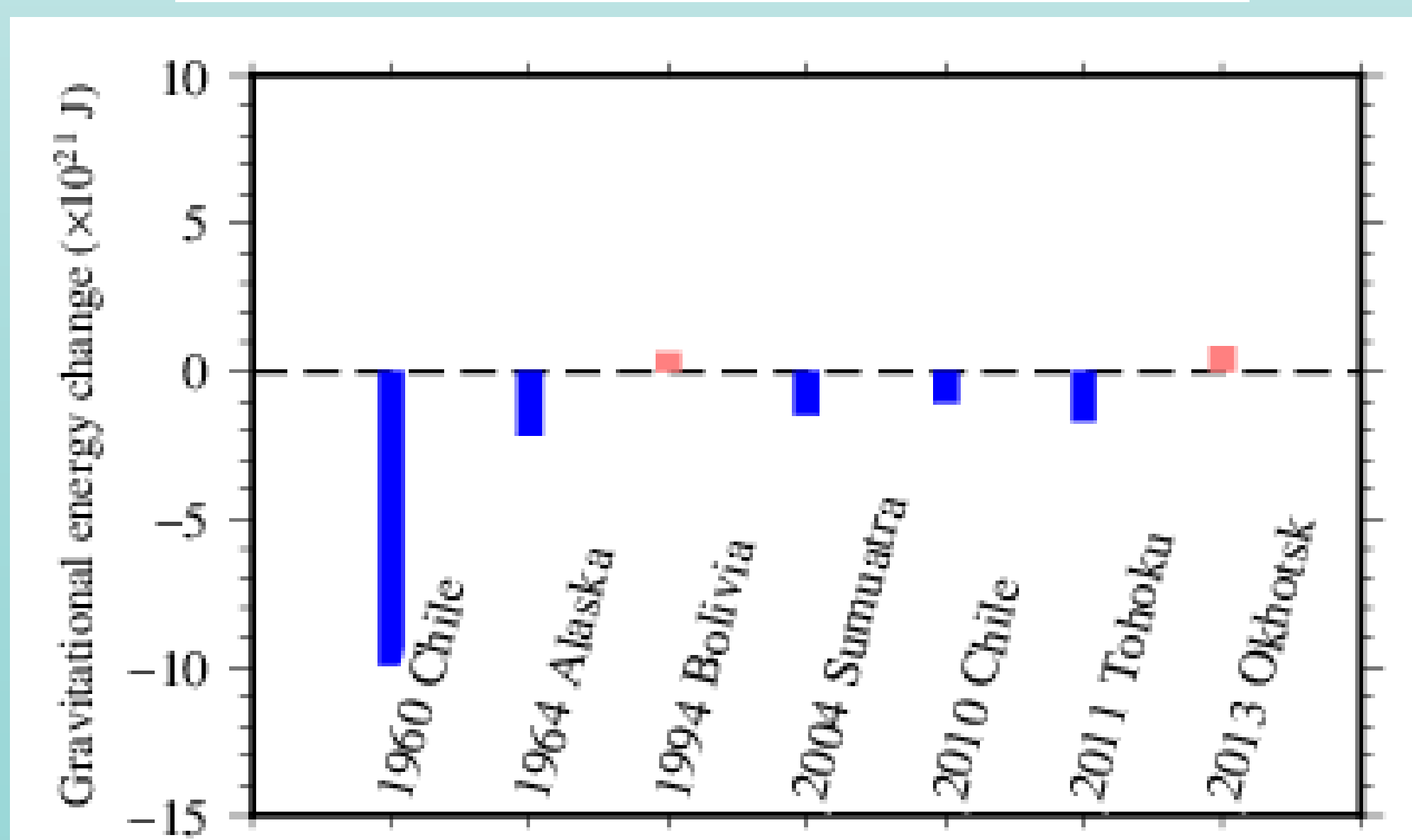
Figure 3: Coseismic gravitational potential energy changes for selected great earthquakes.
