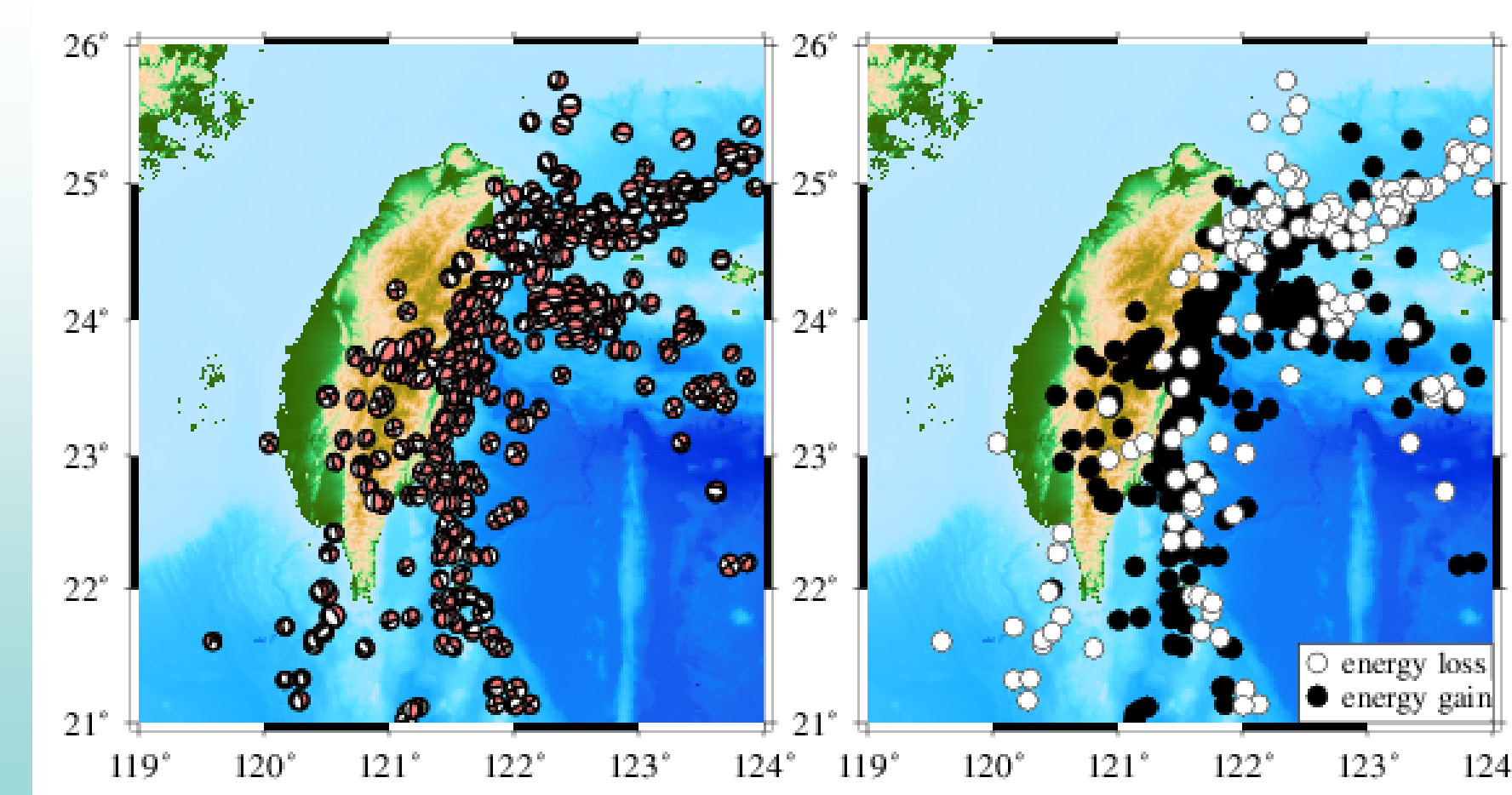
Figure 8: Tectonic signature revealed by coseismic crustal E_g changes
