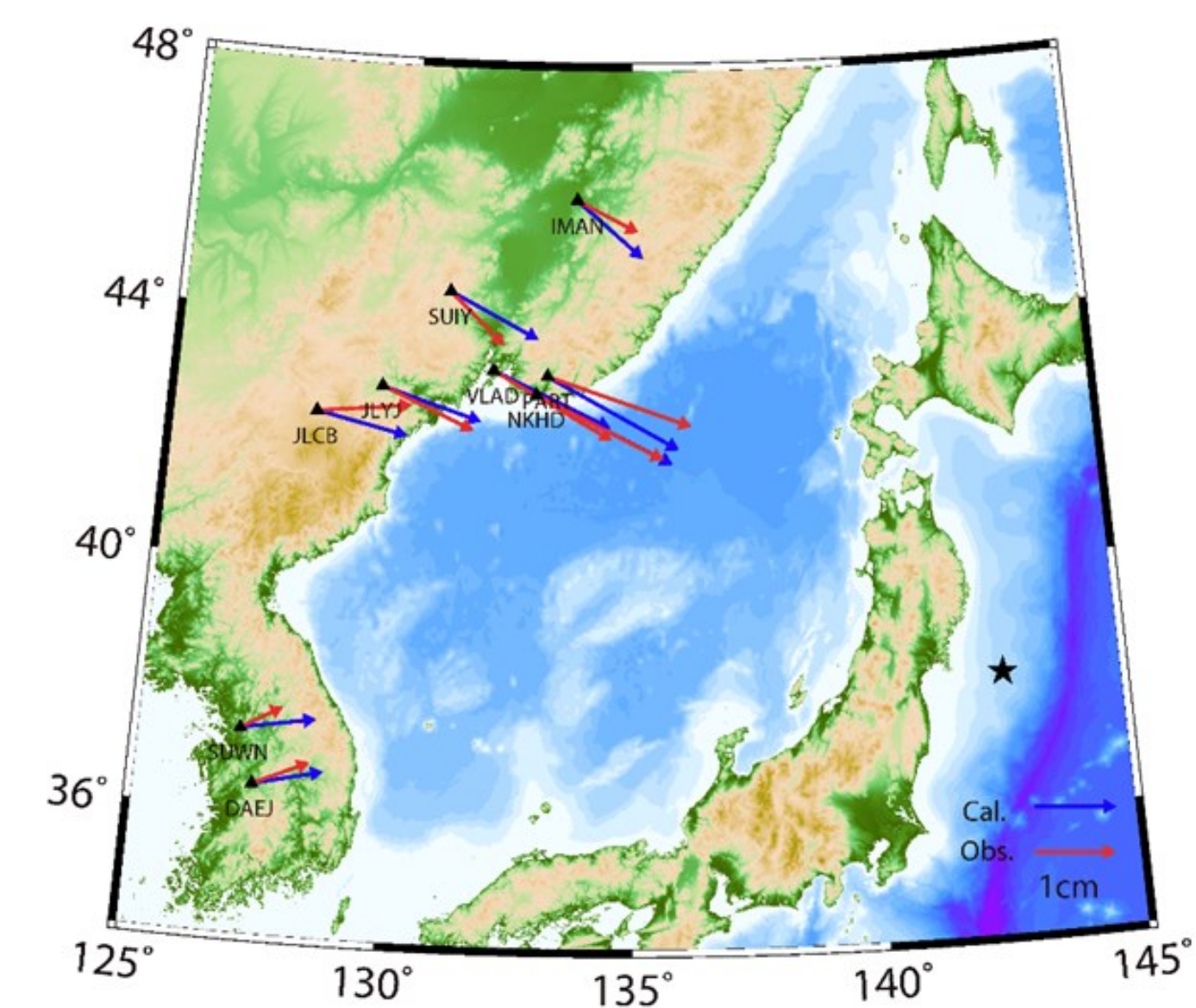
Figure 2 Comparison between accumulated post-seismic deformations observed from nine far-field GPS stations and modeled from 2.5 to 4.5 years after the Mw9.0 earthquake. The red arrows indicate the GPS results; the blue arrows show the fitted results from the viscoelastic spherical dislocation theory at a viscosity of 1 \times 10^{19} Pa·s
